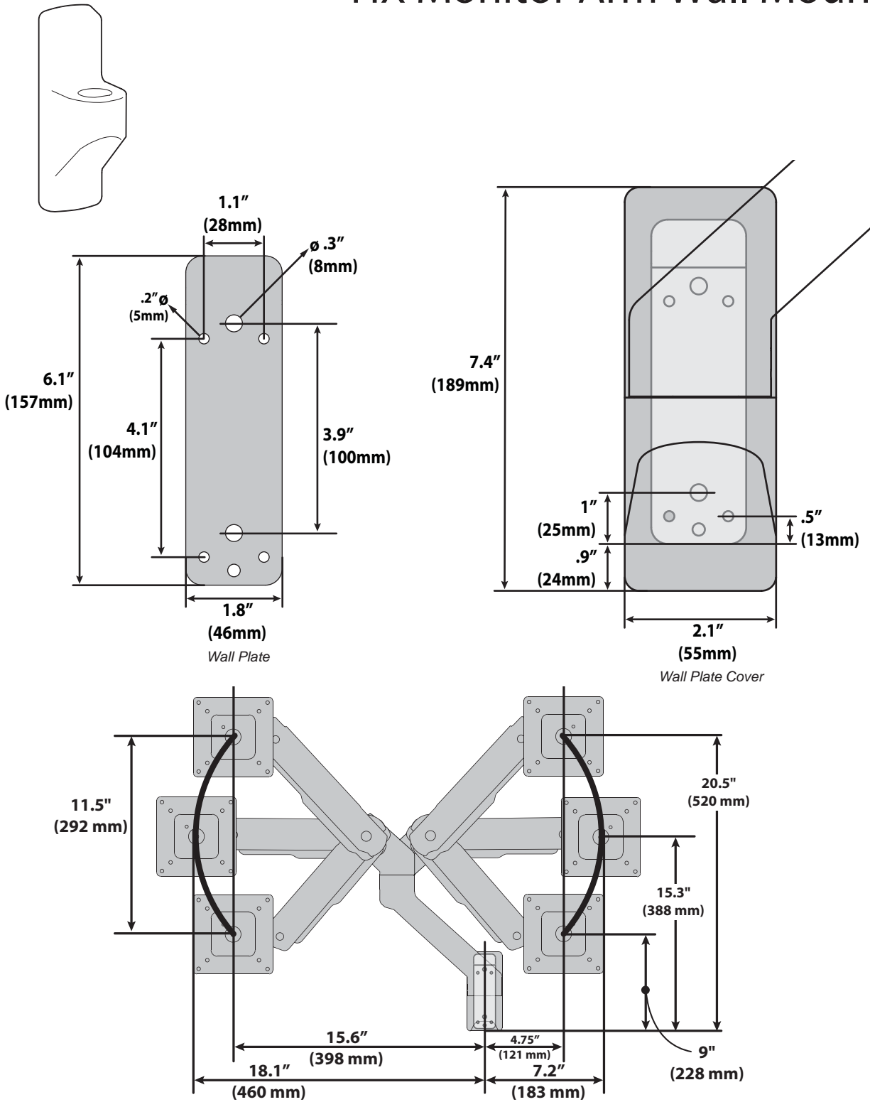
Front View
