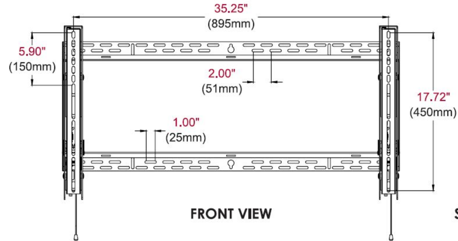
WALL PLATE DETAIL
