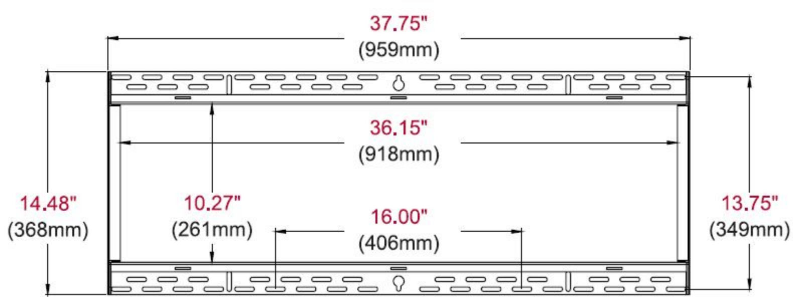
WALL PLATE DETAIL
