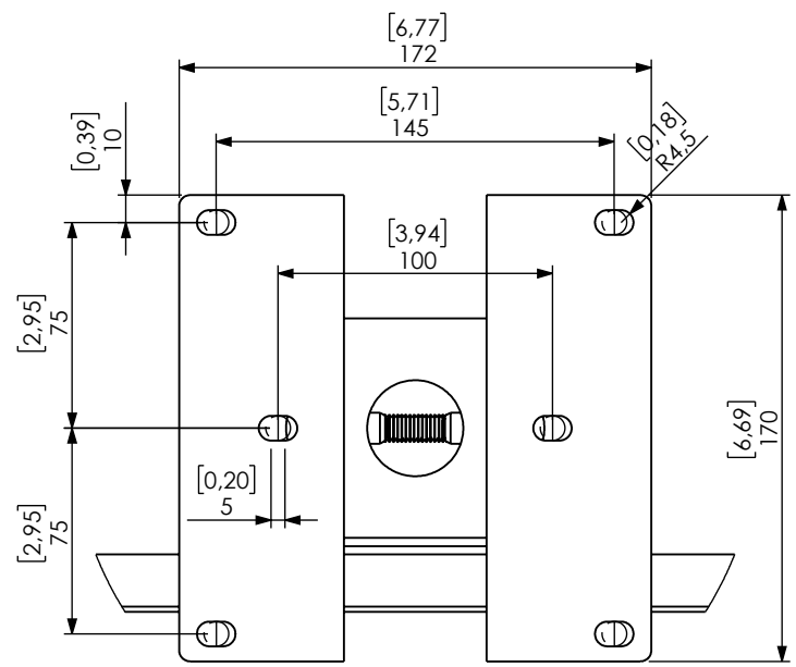
DETAIL A SCALE 1 : 3
