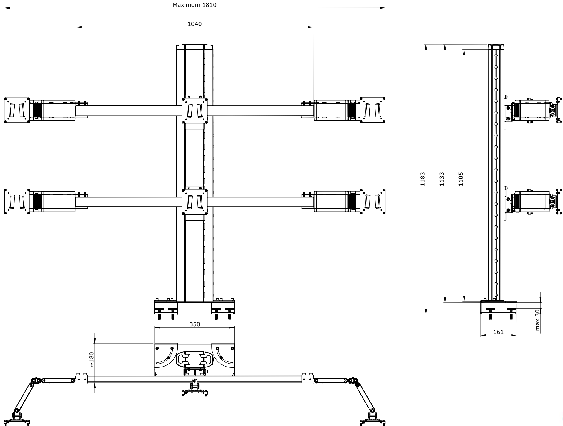
MM051004.P0 SMS Multi Control 2xTriple Clamp dimensinos in mm
