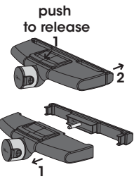
5 Flex Mount
