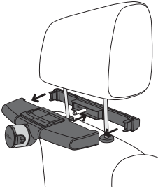
Mount Release
