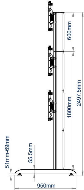
SIDE VIEW
