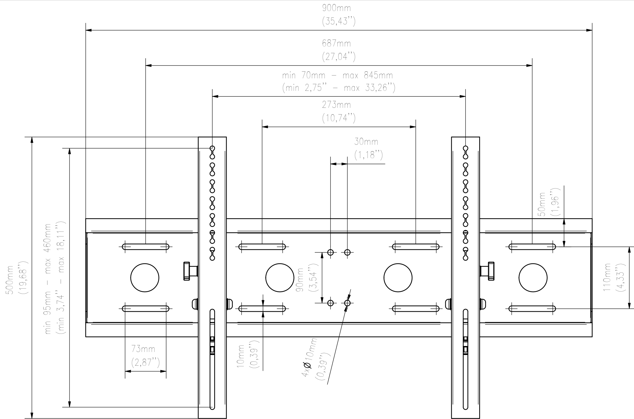
FRONT VIEW
