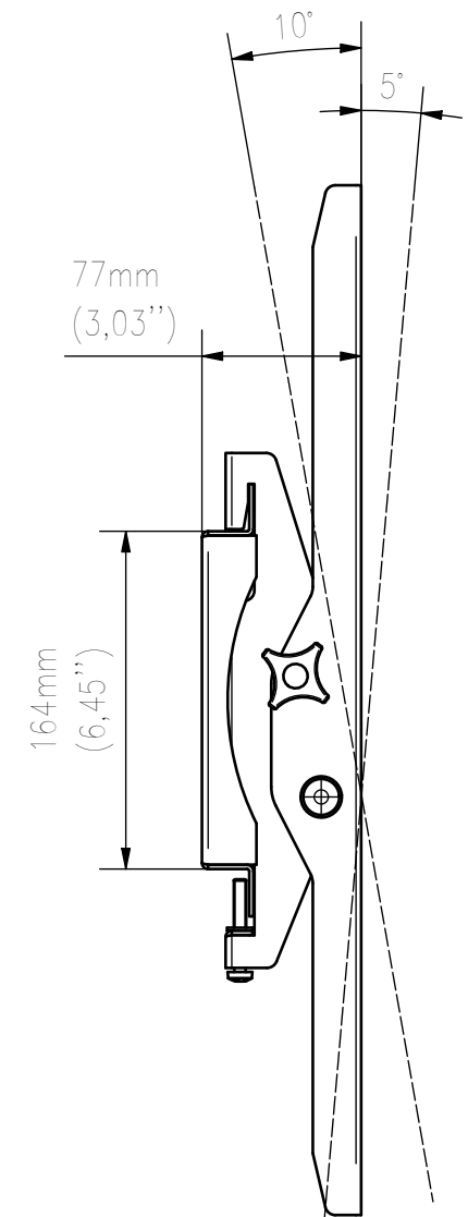
SIDE VIEW
